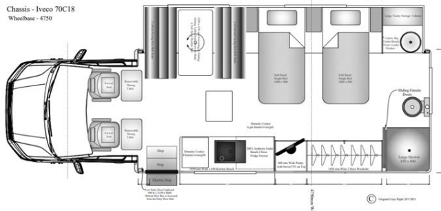
DESIRE 26.5 SL Slide-out Mechanism. Provisional Patent #2018901534
