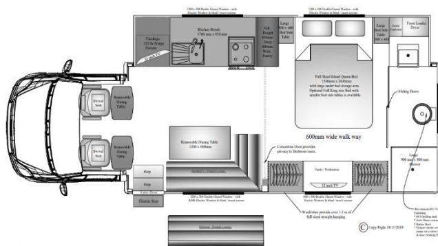
Slide-out. Provisional Patent #2018901534
